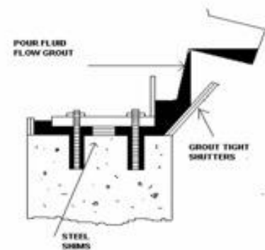
FIGURE 1. GROUT SHUTTER DETAIL
